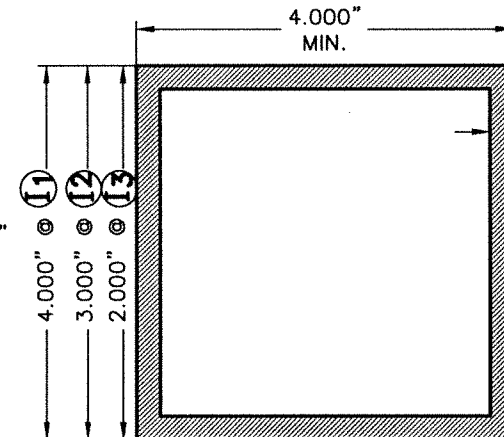
(I, I2, I3) BUILD-OUT MOUNTED TUBE (MASONRY)
