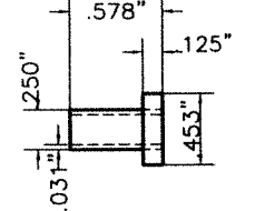
(F) SCREW SLEEVE
