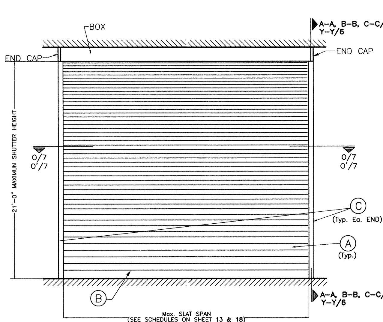
TYPICAL SINGLE UNIT ELEVATION (CONCRETE, GROUTED BLOCK OR WOOD)
