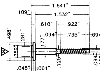
(E) WIND LOCK SCREW
